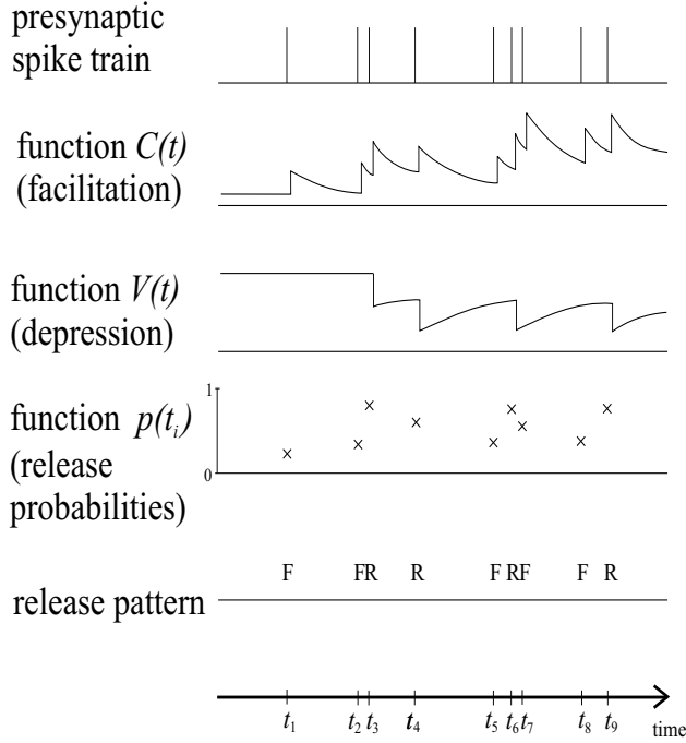
Figure 5: Synaptic computation on a spike train \underline{t} , together with the temporal dynamics of the internal variables C and V of our model. Note that V(t) changes its value only when a presynaptic spike causes release.
